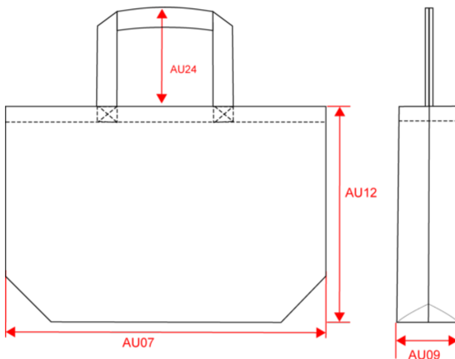
Dimensions (cm)
